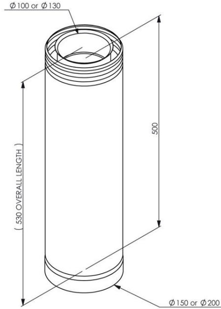
2 US 50 100 ( \phi 100 ) US 50 130 ( \phi 130 ) Length 500mm
