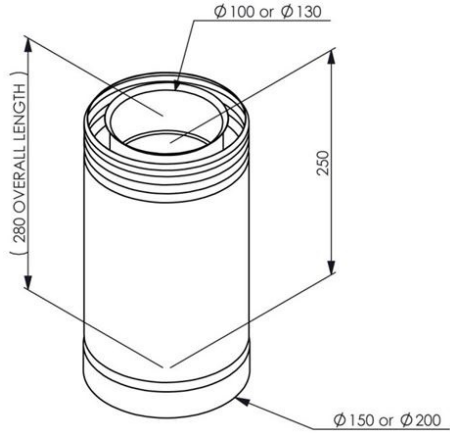
1 US 25 100 ( \phi 100 ) US 25 130 ( \phi 130 ) Length 250mm
